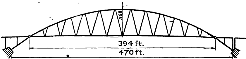
Fig. 372.—Bridge over River Lot at Castlemoron, France.
